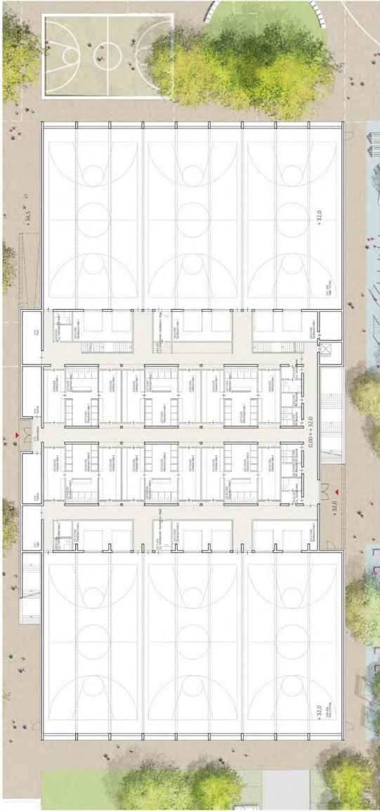
ERDGESCHOSS SPORTHALLE M 1:200
